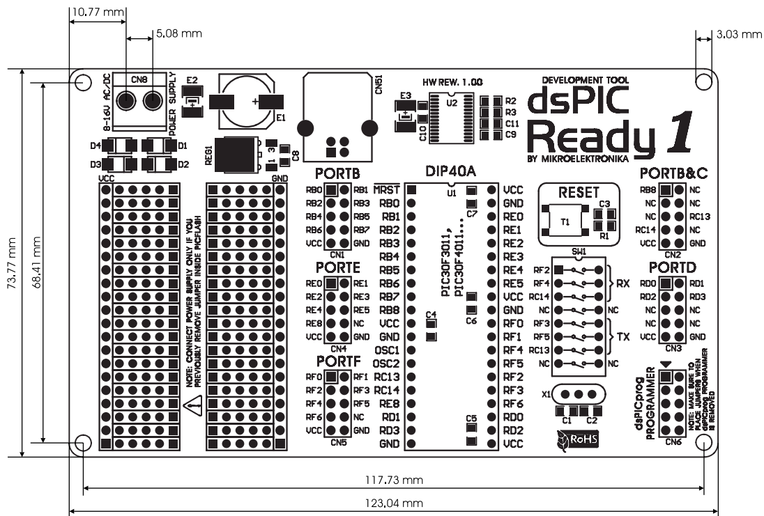
Figure 4: Dimensions of the dsPIC Ready1 additional board
