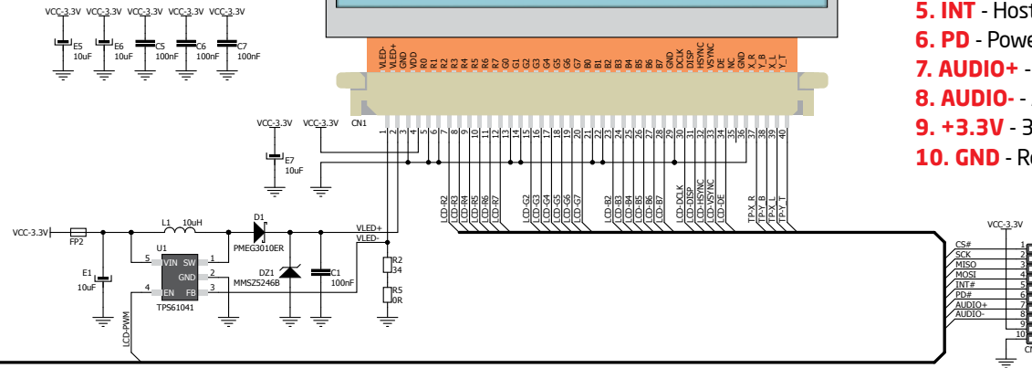
Figure 2: ConnectEVE schematic
