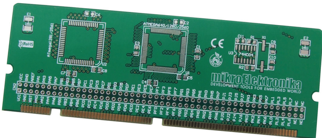
Figure 7: Empty 64/100 pin MCU card MCU Card 2
