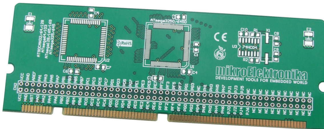
Figure 6: Empty 64/100 pin MCU card MCU Card 1
