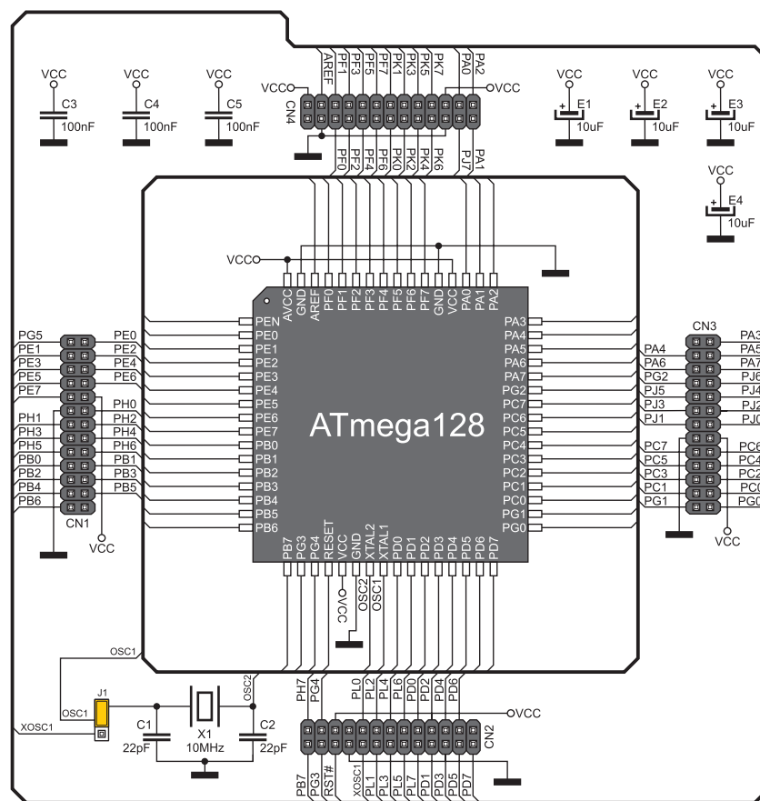
Figure 1: 64-pin MCU card and microcontroller connection schematic
