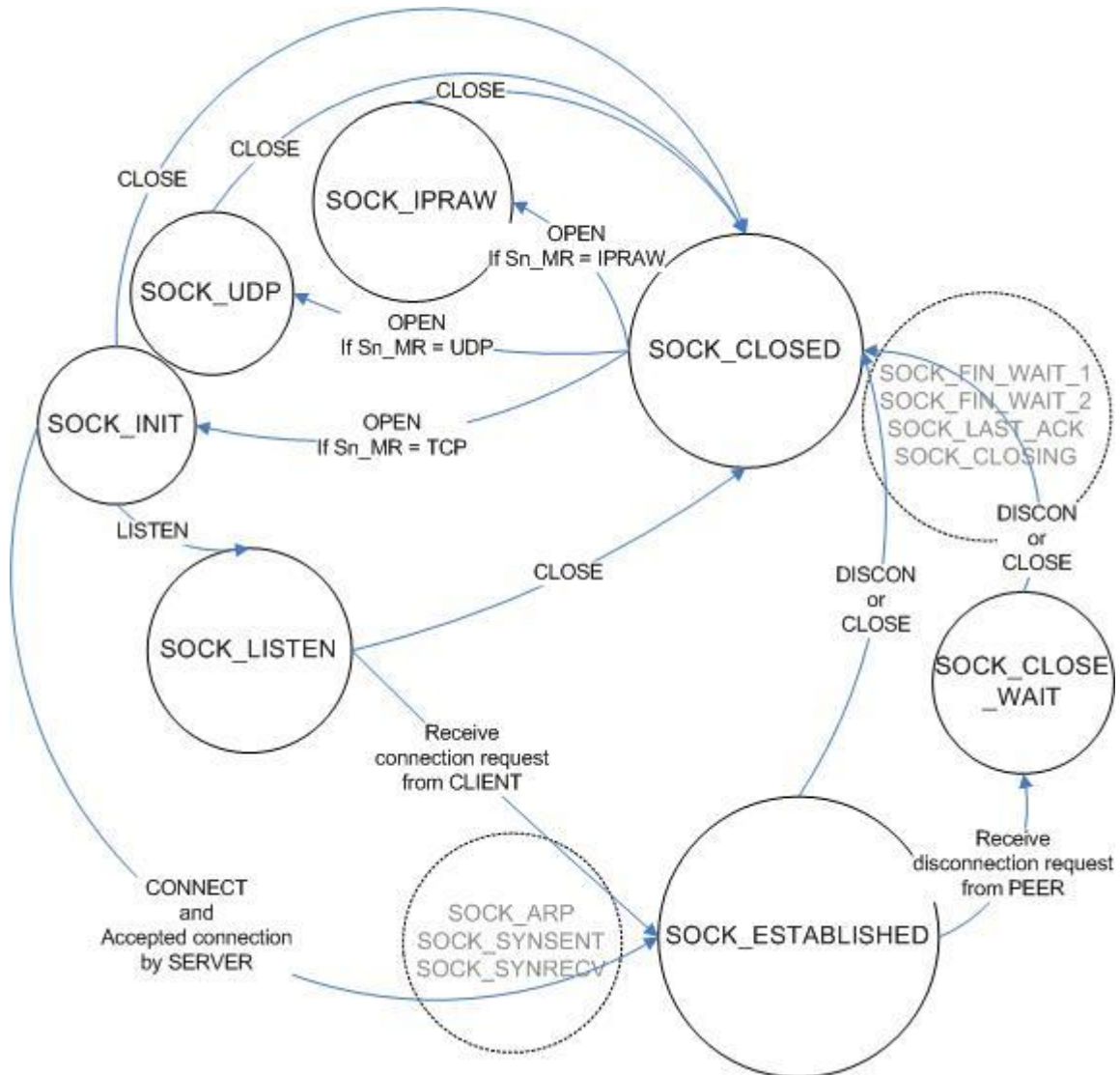
Figure 4-1. State Diagram
