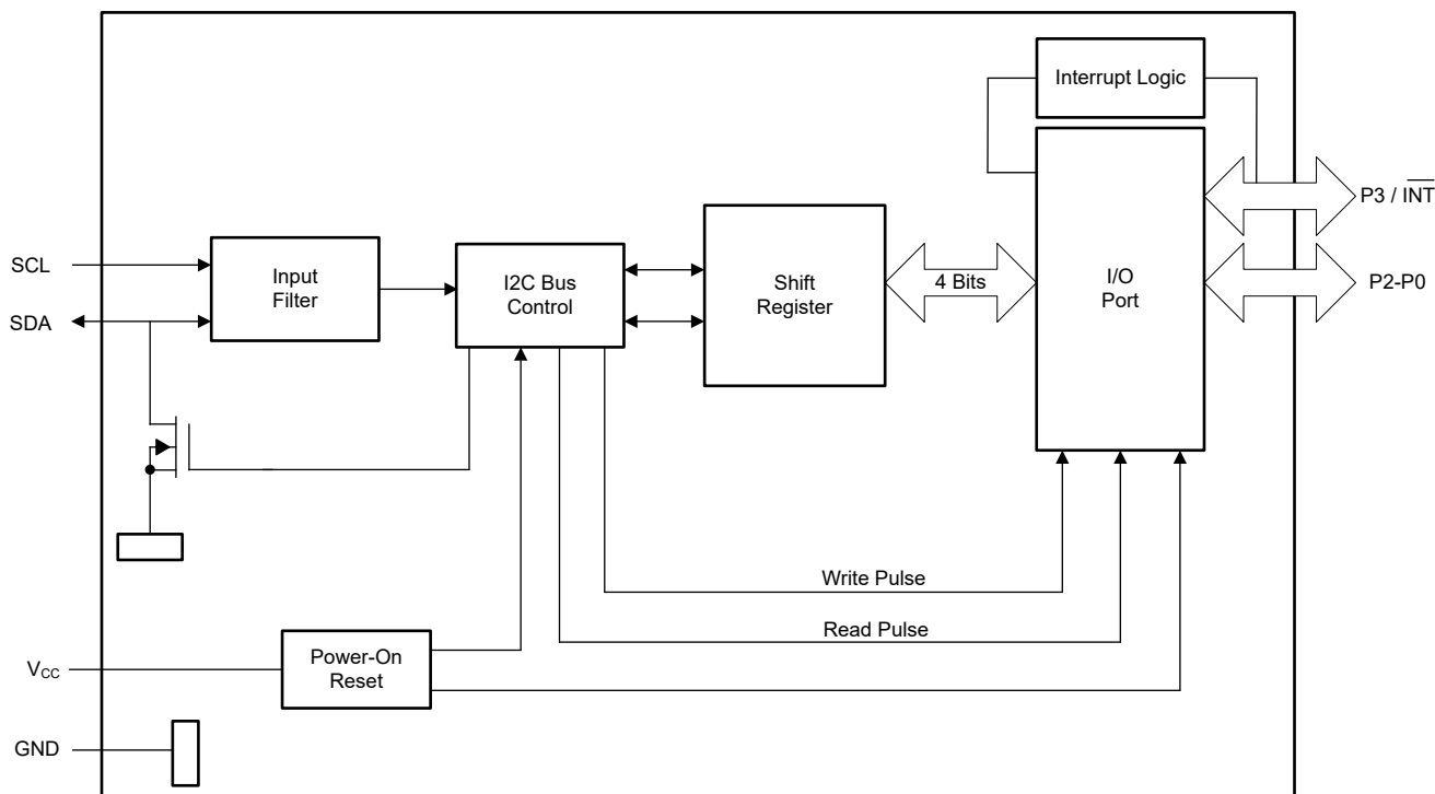
Figure 8-1. Logic Diagram
