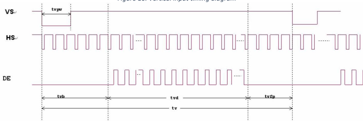
Figure 10. Vertical input timing diagram
