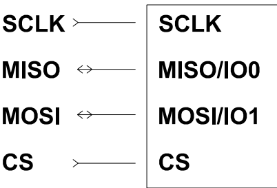
Figure 4.SPI interface connection
