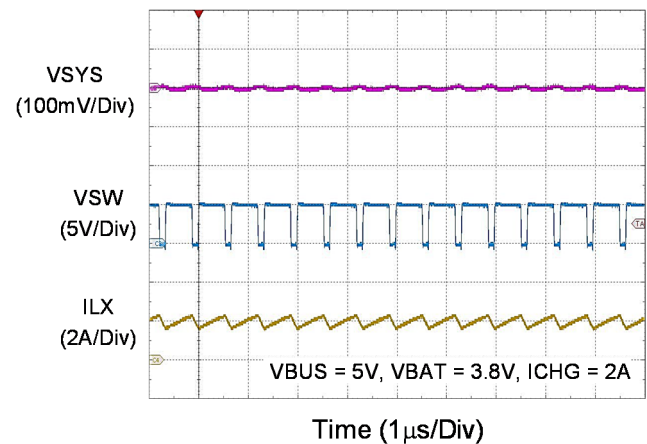
Buck Switching
