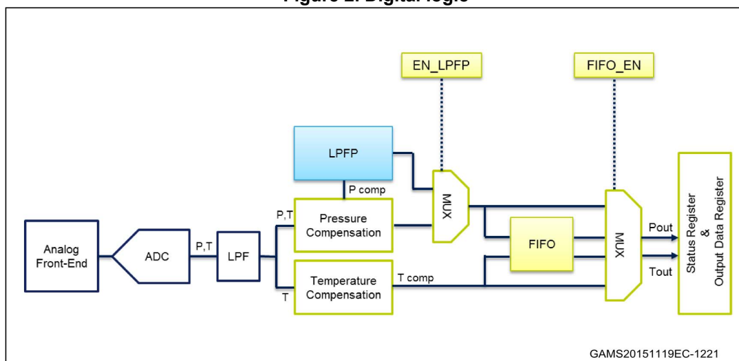
Figure 2. Digital logic
