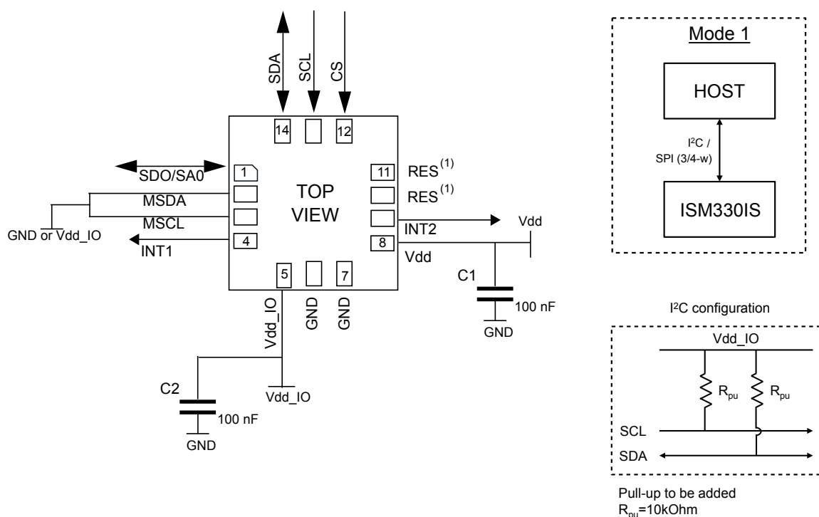
Figure 15. ISM330IS electrical connections in mode 1
