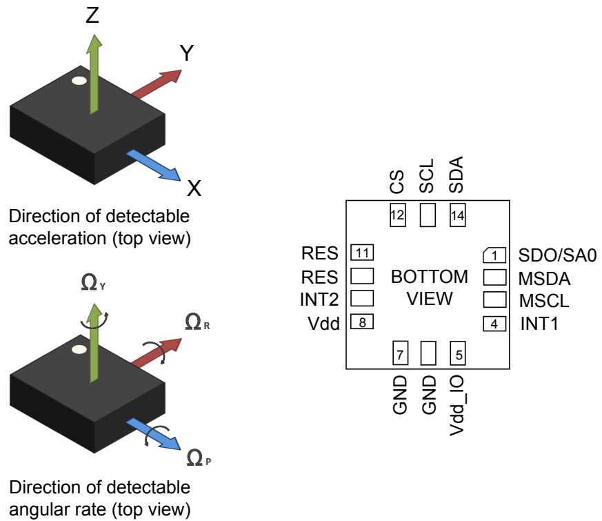
Figure 2. Pin connections
