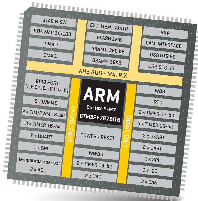
Figure 1: STM32F767BI MCU block schematic
