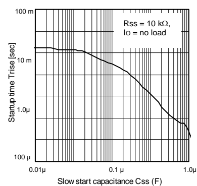
Fig.24 Soft Start Rise Time (BH30PB1WHFV)
