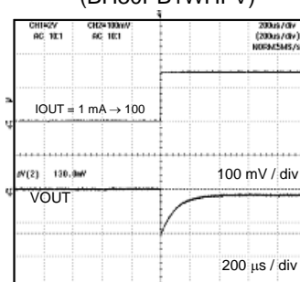
Fig.21 Load Response (Co=1.0 μF) (BH30PB1WHFV)
