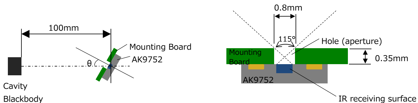
Figure 15.2. Measurement environment
