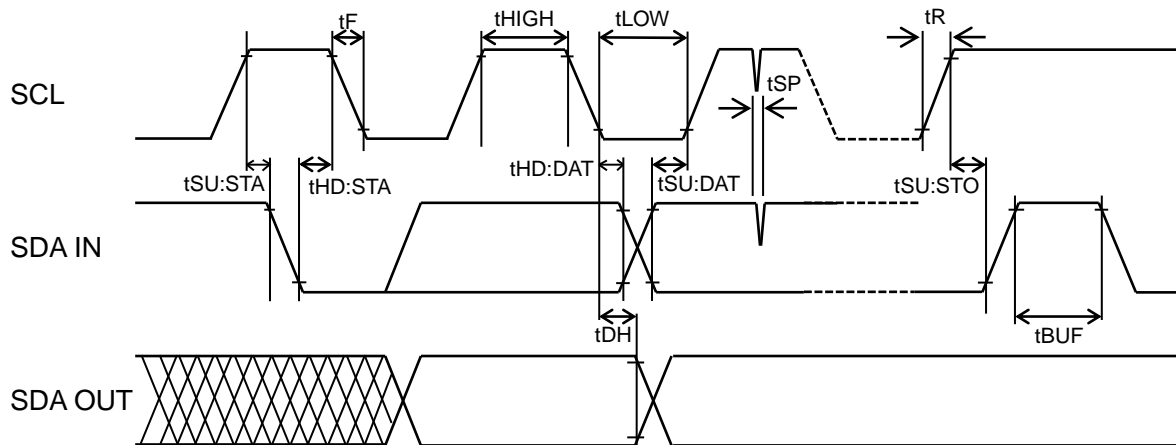
Figure 9.1 Bus Timing
