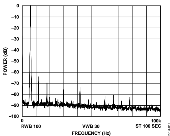
Figure 17. Power vs. Frequency, f_{MCLK} = 25 MHz, f_{OUT} = 6 kHz, Frequency Word = 0x000FBA9
