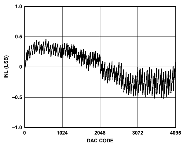
Figure 13. DAC INL
