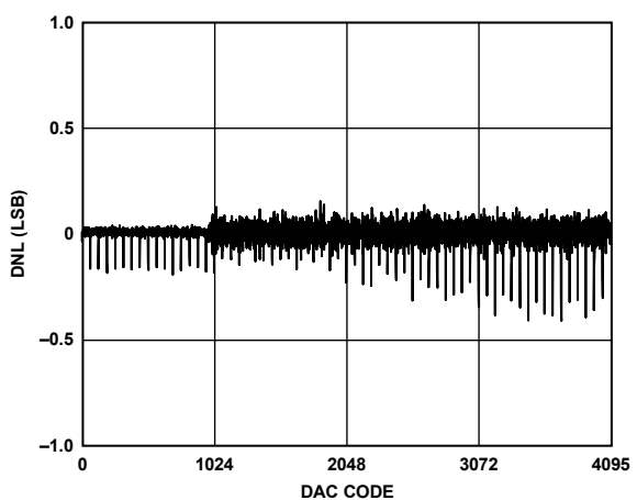
Figure 14. DAC DNL
