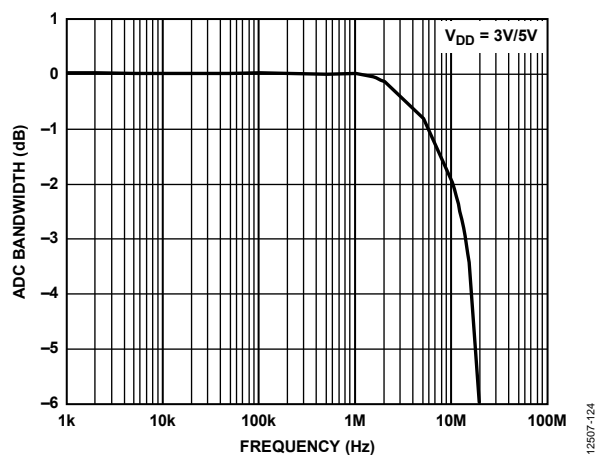
Figure 12. ADC Bandwidth
