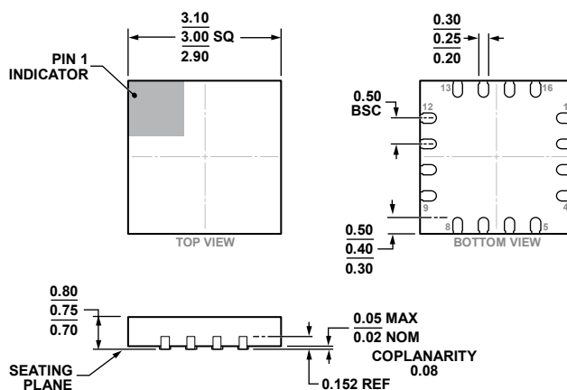
Figure 43. 16-Lead Lead Frame Chip Scale Package [LFCSP] 3 mm × 3 mm Body and 0.75 mm Package Height (CP-16-32)
