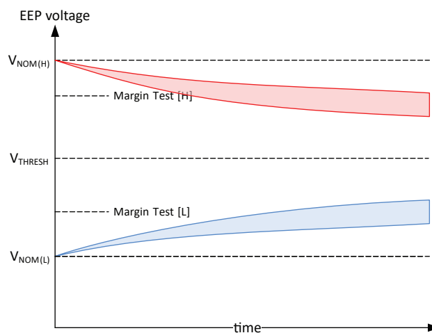
Figure 30: Example of passing programming voltages
