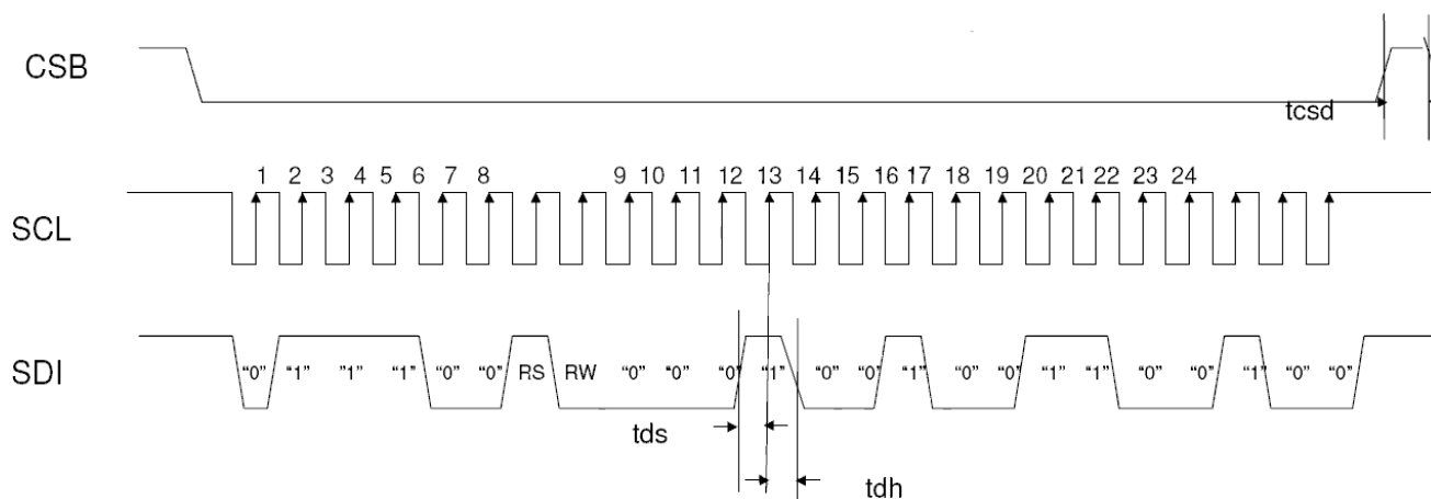
Figure 14. 12 SPI interface Timing Diagram & Transaction Example
