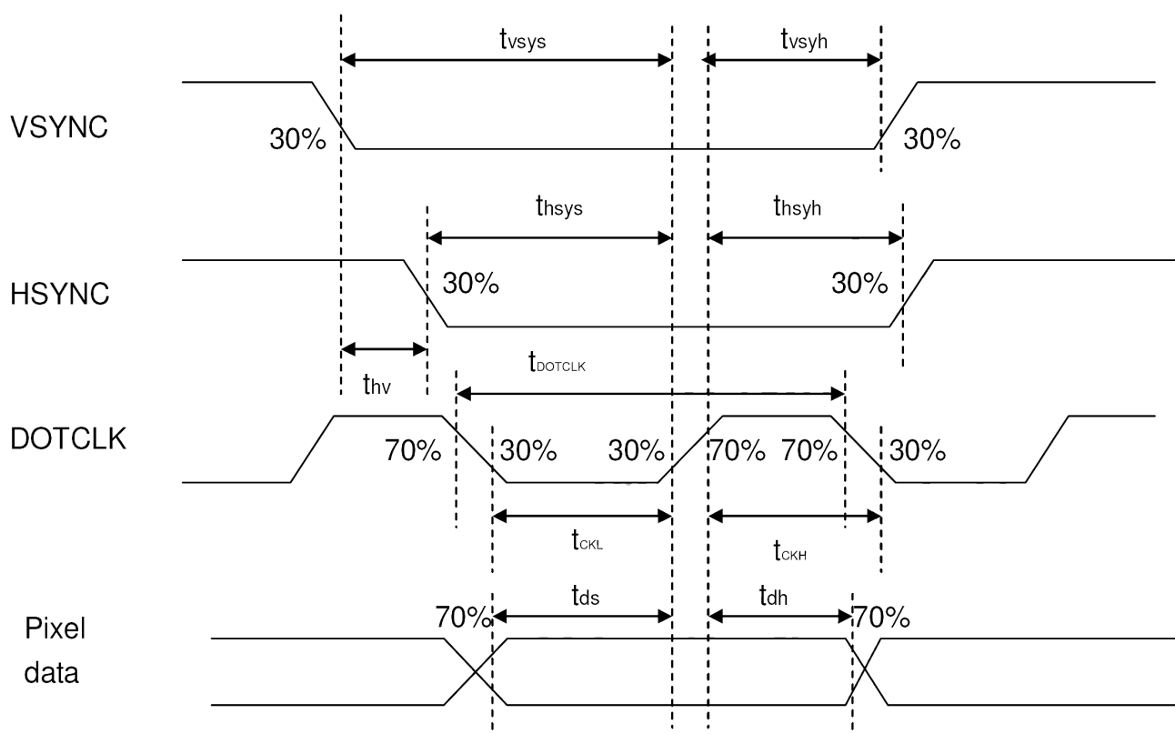
Figure 13. 1Pixel Timing
