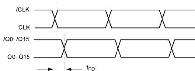
Propagation Delay
