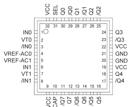
32-Pin QFN
