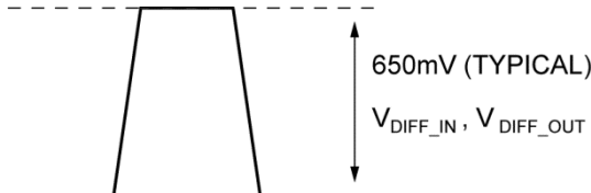
Figure 5. Differential Swing
