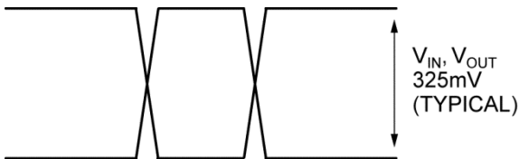
Figure 4. Single-Ended Swing
