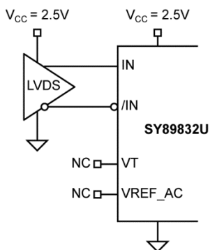
Figure 10. LVDS Input Interface
