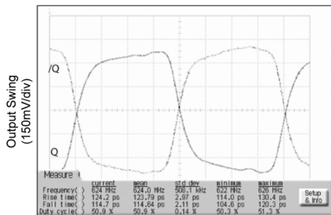
622MHz Output
