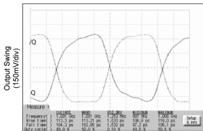
1GHz Output
