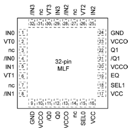
32-Pin QFN
