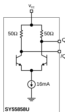
Figure 2. Output Stage
