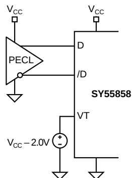
Figure 5c. PECL-to-CML (DC-Coupled) Input Interface
