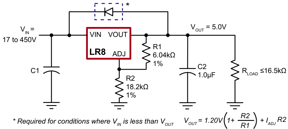
Figure 1: High Input Voltage, 5.0V Output Linear Regulator
