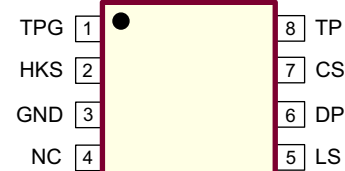
8-Lead SOIC (Narrow Body) (LG) (top view)
