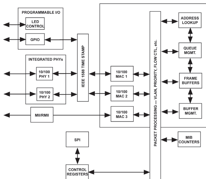
KSZ8463MLI / RLI
