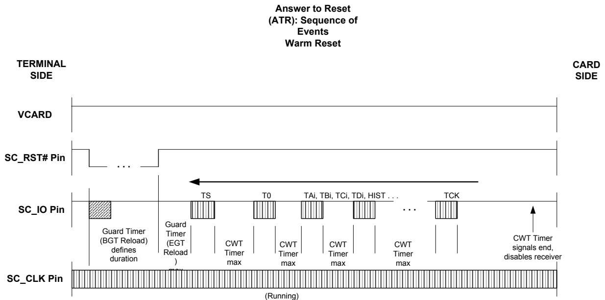
Figure 13.9 ATR Sequence, Warm Reset
