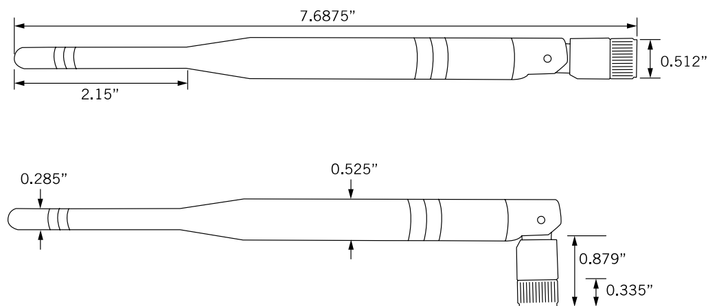
Figure 1. Antenna Dimensions
