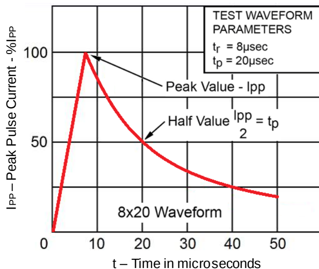
FIGURE 2 Pulse Waveform
