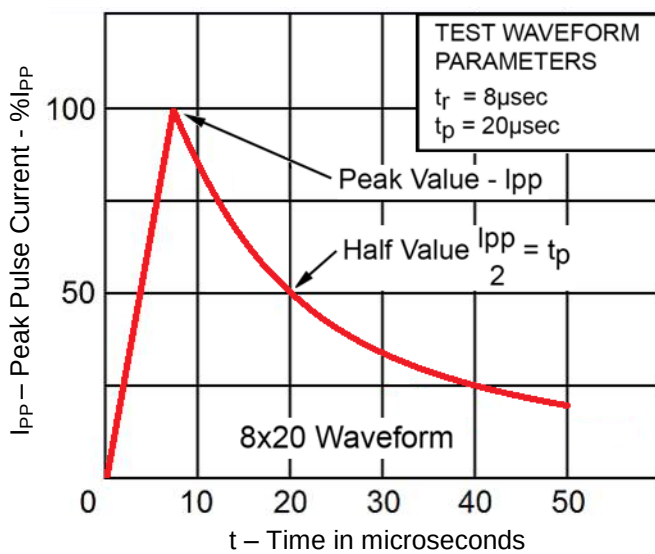
FIGURE 2 Pulse Waveform
