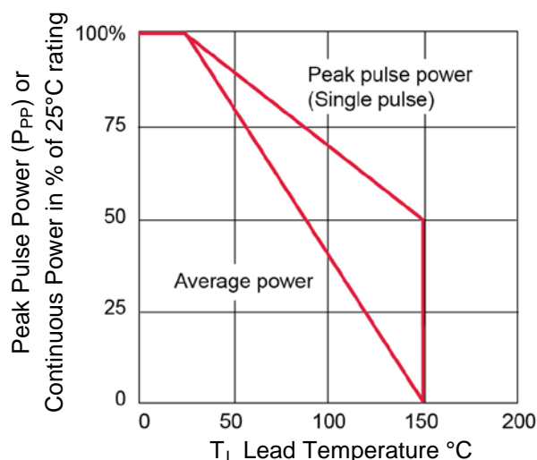
FIGURE 2 Power Derating
