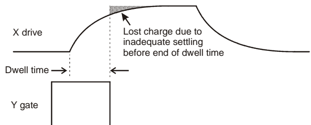
Figure 2.4 X-Drive Pulse Roll-off and Dwell Time The Dwell time is fixed at ~500ns - see Section 2.7
