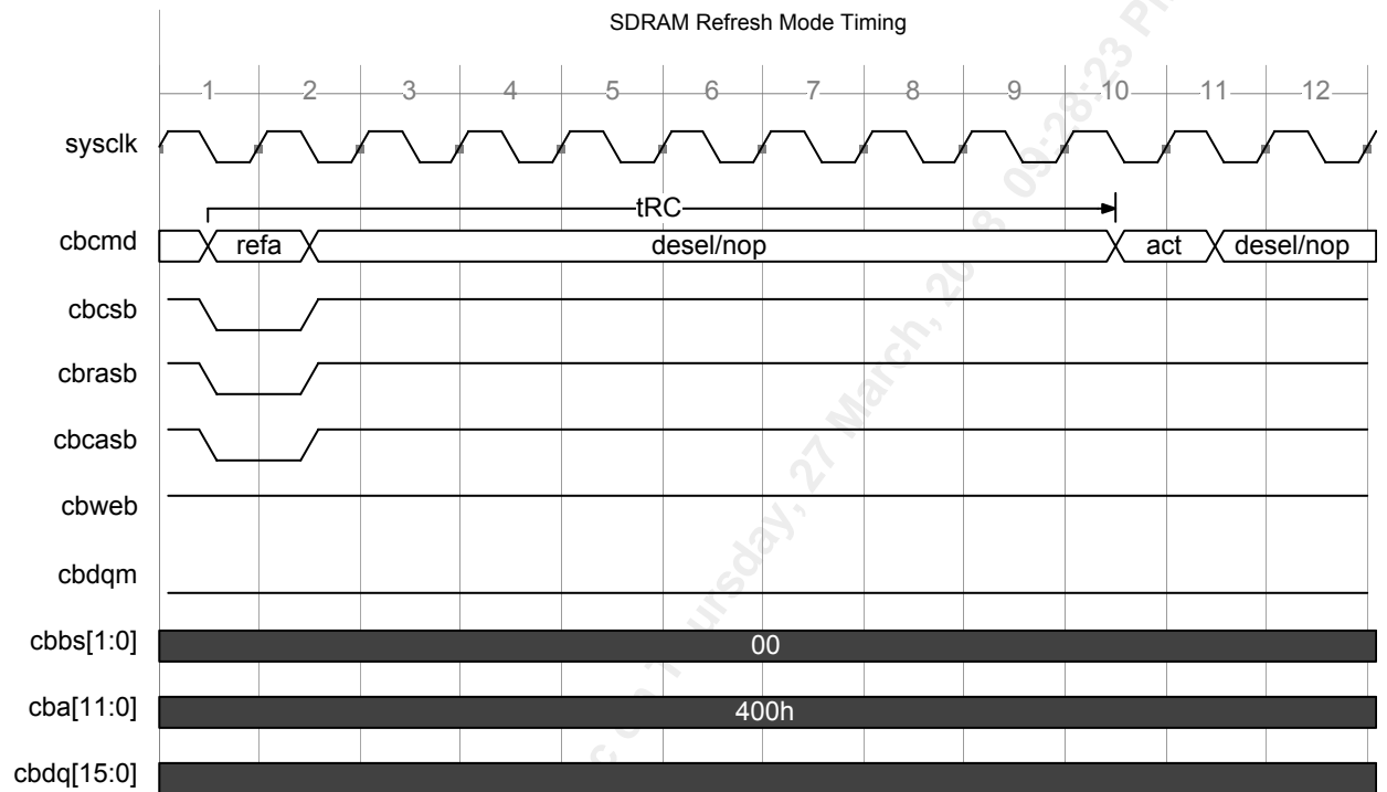
Figure 48 SDRAM Refresh
