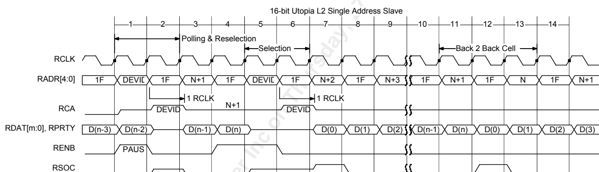
Figure 44 UTOPIA L2 Single-PHY Receive Slave
