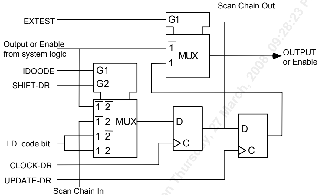
Figure 31 Bi-directional Cell (IO_CELL)
