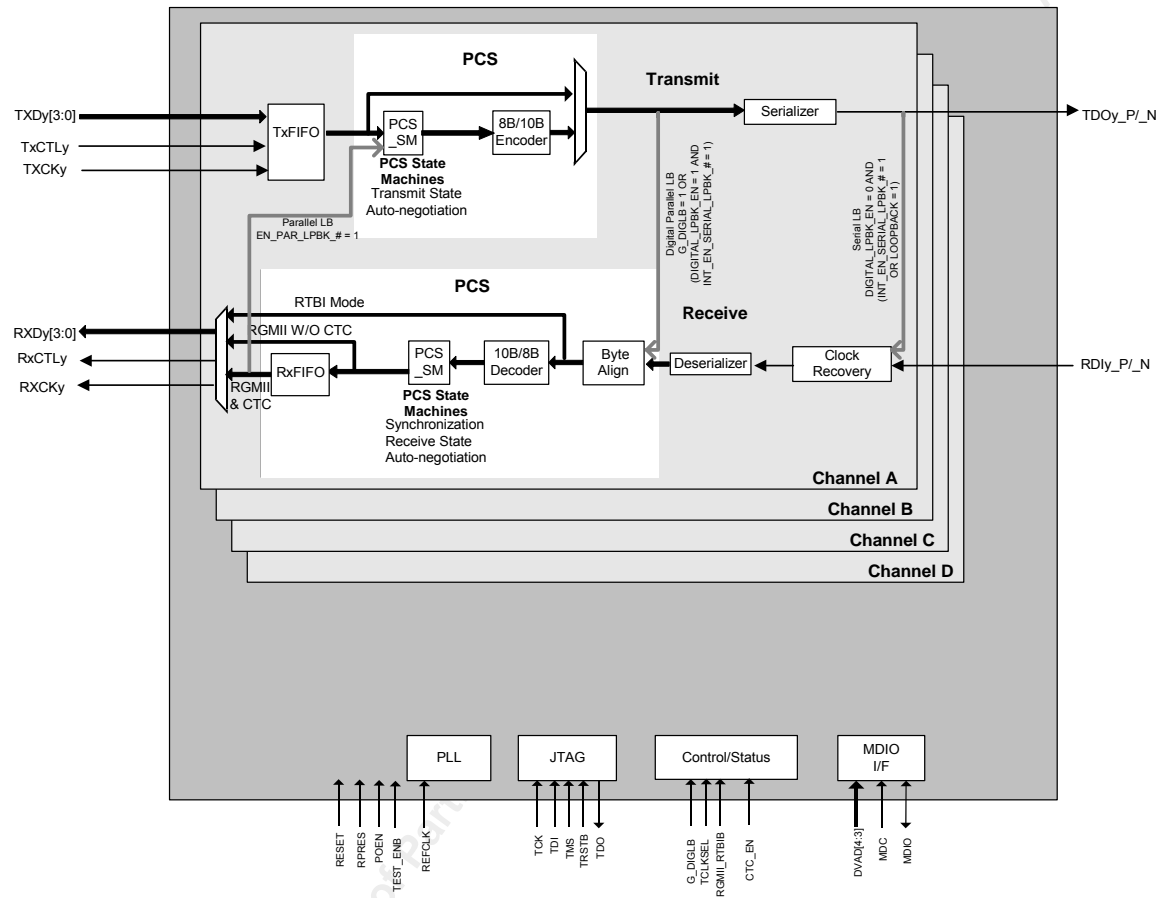
Figure 4 QuadPHY 1GR Loopback Diagram
