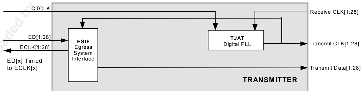
Figure 18 - Clock Master: Clear Channel
