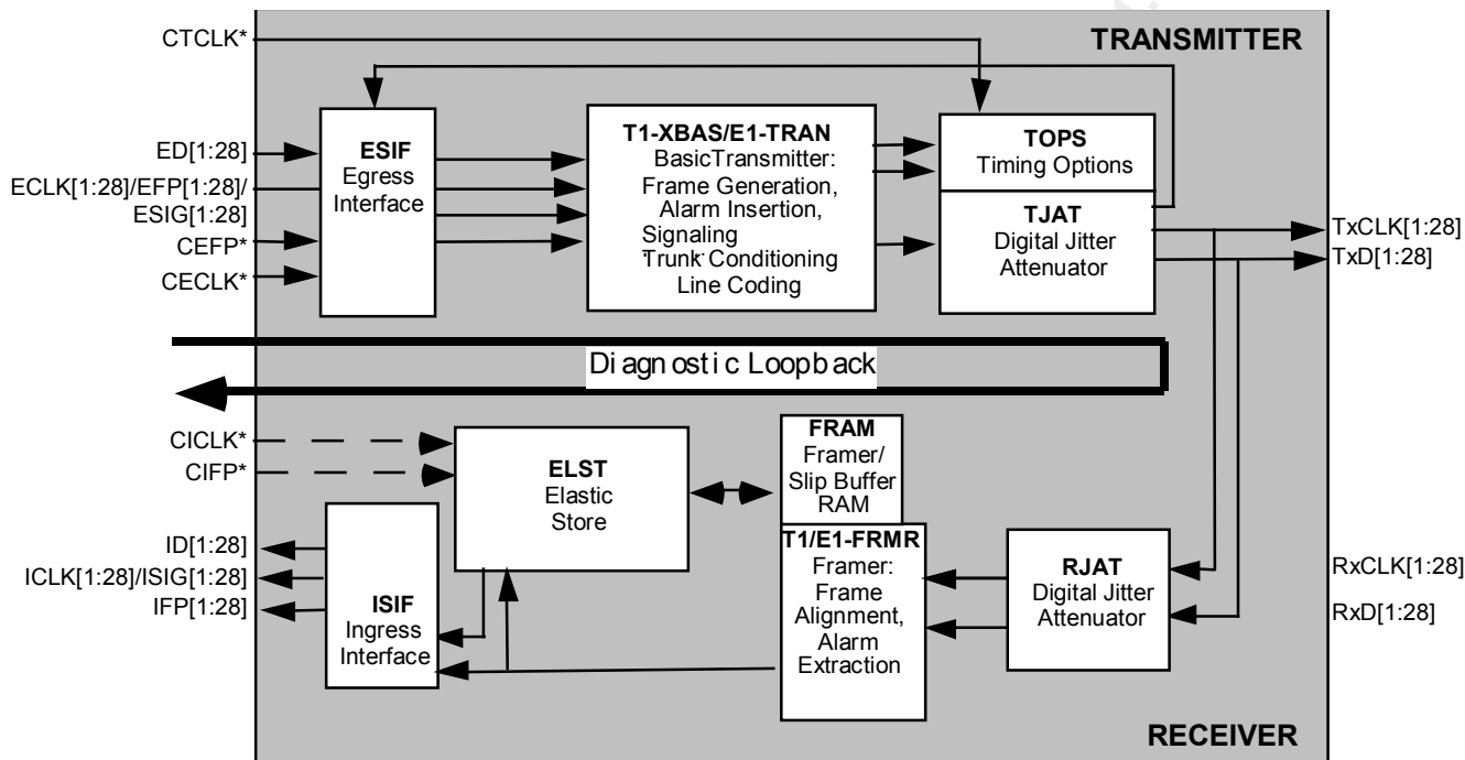
Figure 40 - T1/E1 Diagnostic Digital Loopback
