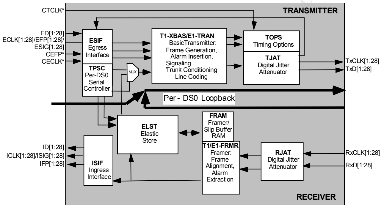
Figure 41 - Per-Channel Loopback
