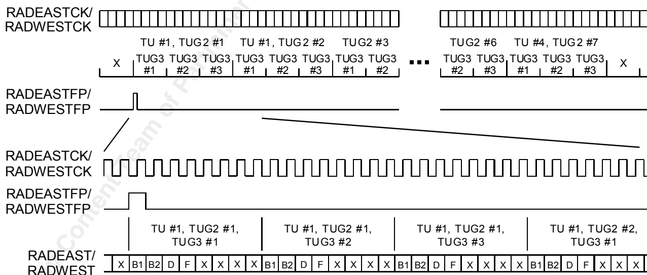
Figure 67 - Remote Serial Alarm Port Timing
