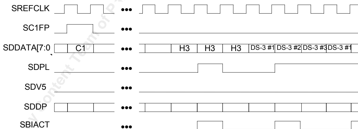
Figure 69 - SBI DROP Bus DS3 Functional Timing
