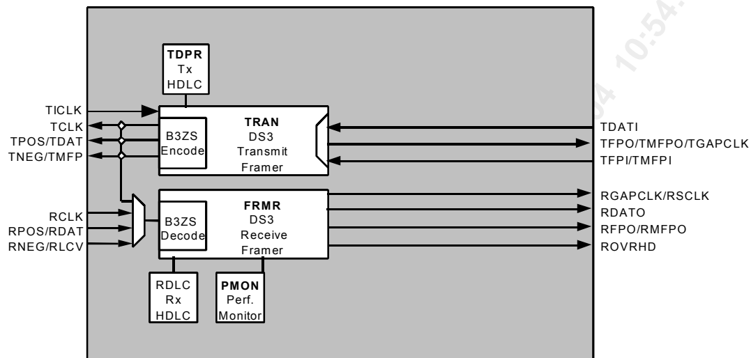
Figure 6 - DS3 Framer Only Mode Block Diagram
