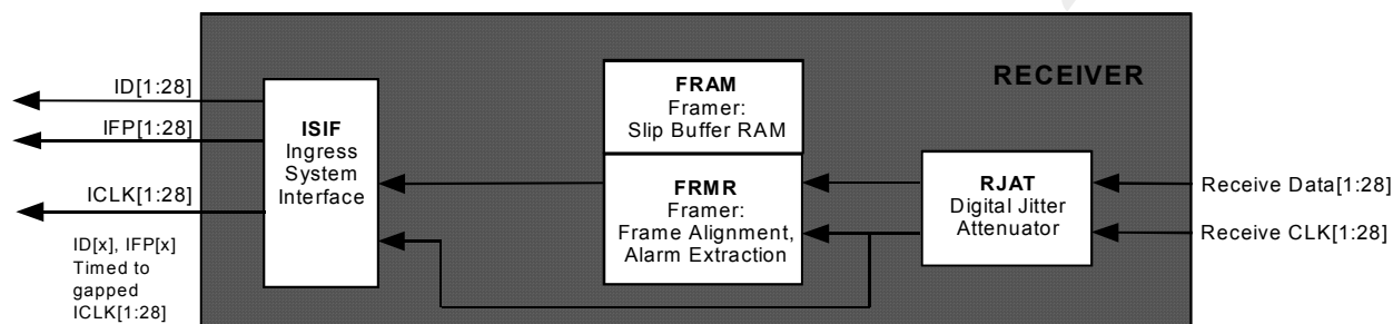
Figure 25 - Clock Master: NxChannel
