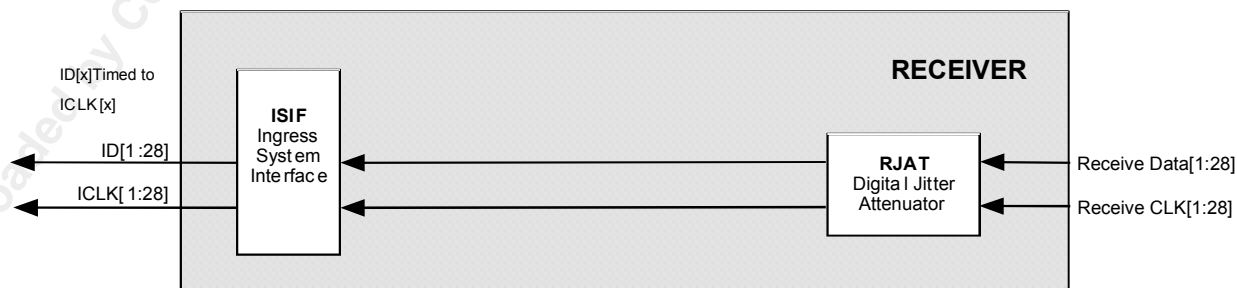
Figure 26 - Clock Master: Clear Channel
