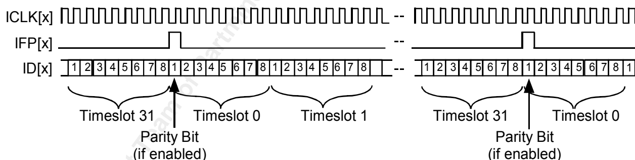
Figure 84 - E1 Ingress Interface Clock Master : Full Channel Mode
