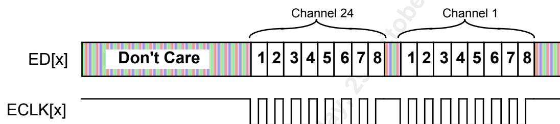
Figure 74 - E1 Egress Interface Clock Master : NxChannel Mode
