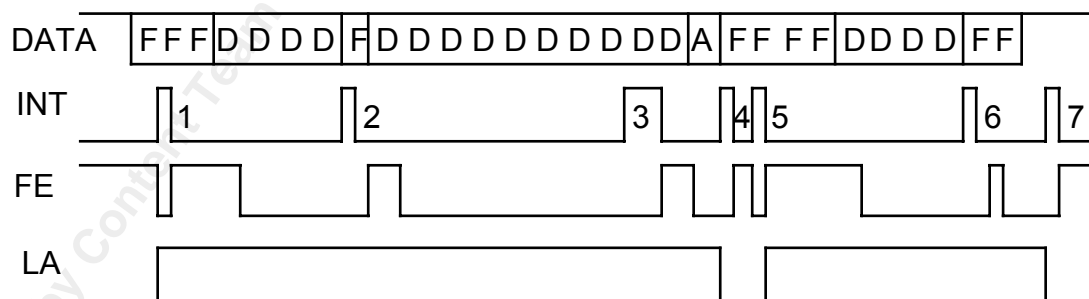
Figure 38 - Example Multi-Packet Operational Sequence
