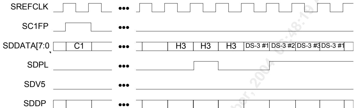
Figure 72 SBI DROP Bus DS3/E3 Functional Timing
