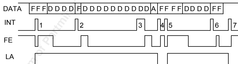
Figure 34 Example Multi-Packet Operational Sequence
