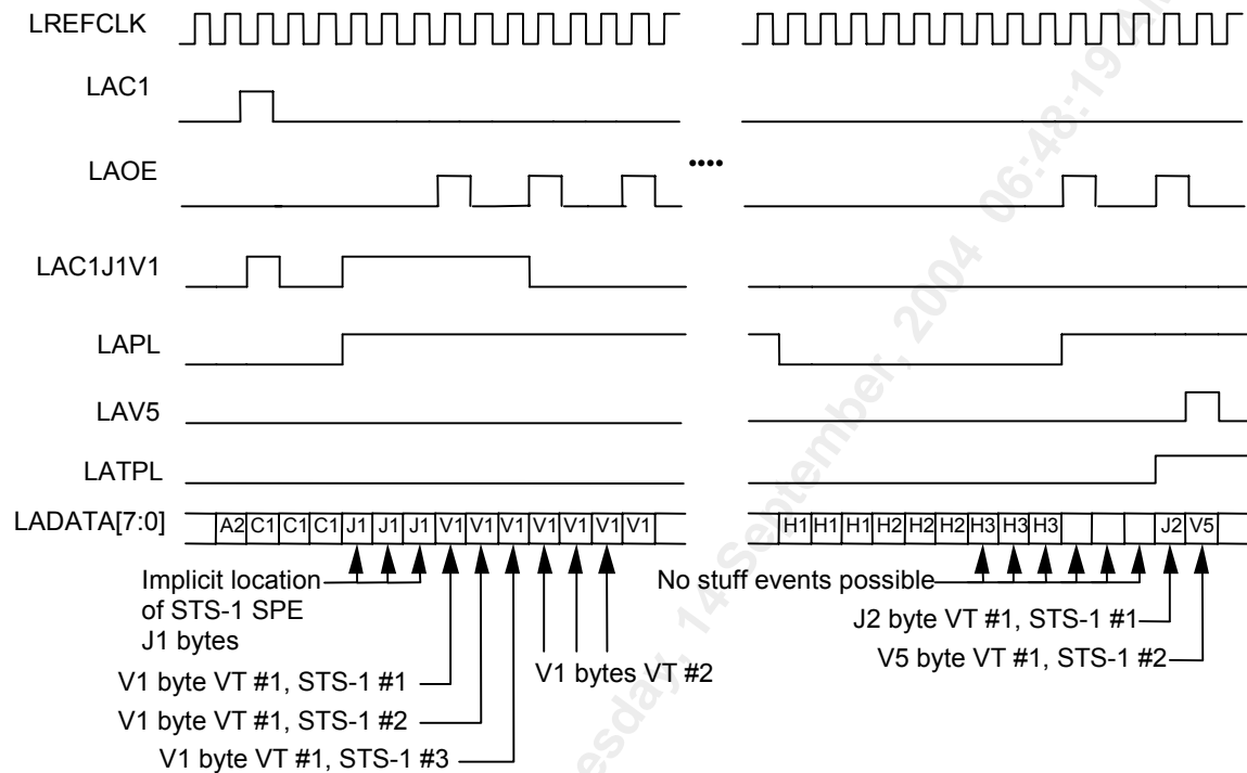
Figure 67 19.44 MHz Telecom ADD Bus Timing - Locked STS-1 SPEs / AU3 VCs
