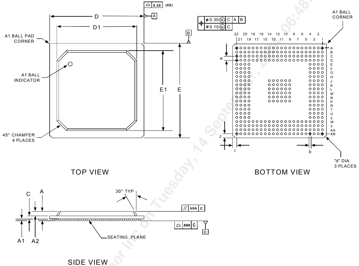
Figure 98 324 Pin PBGA 23x23mm Body
