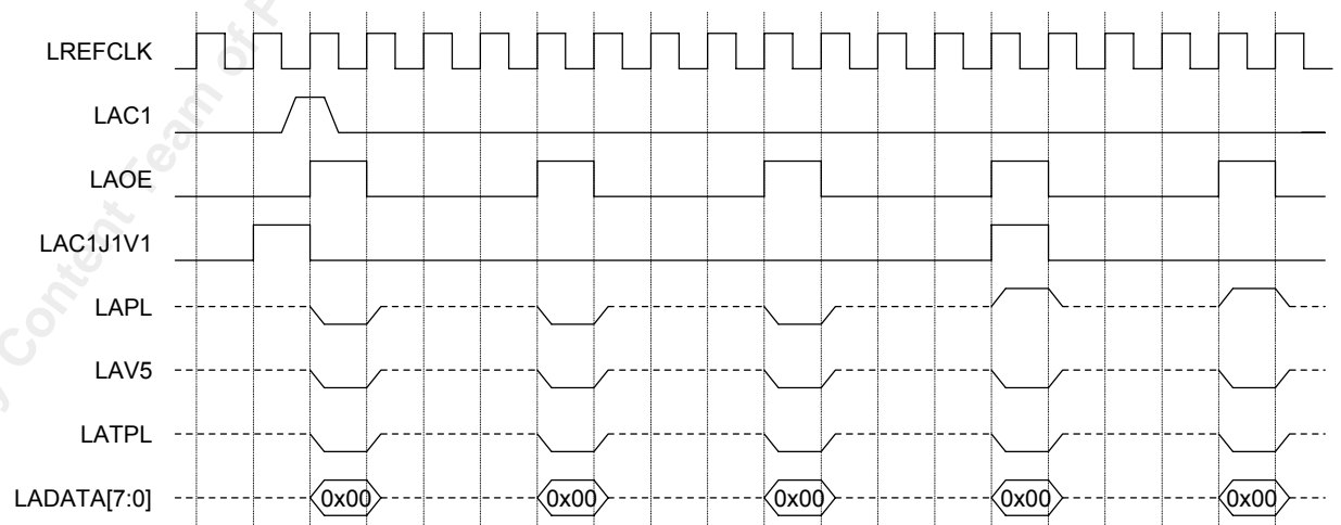
Figure 69 77.76 MHz Telecom ADD Bus Timing
