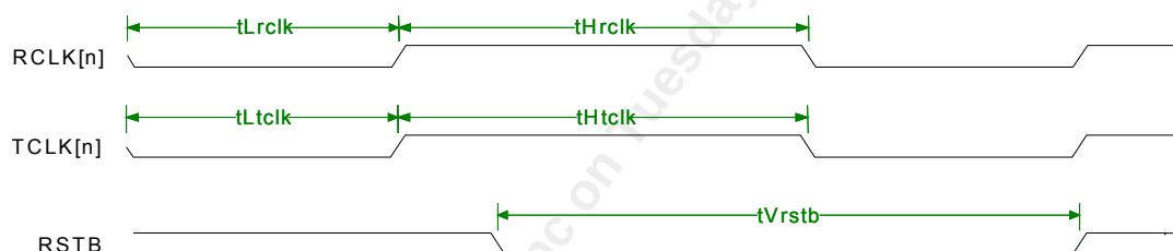
Figure 27 System Miscellaneous Timing Diagram Timing
