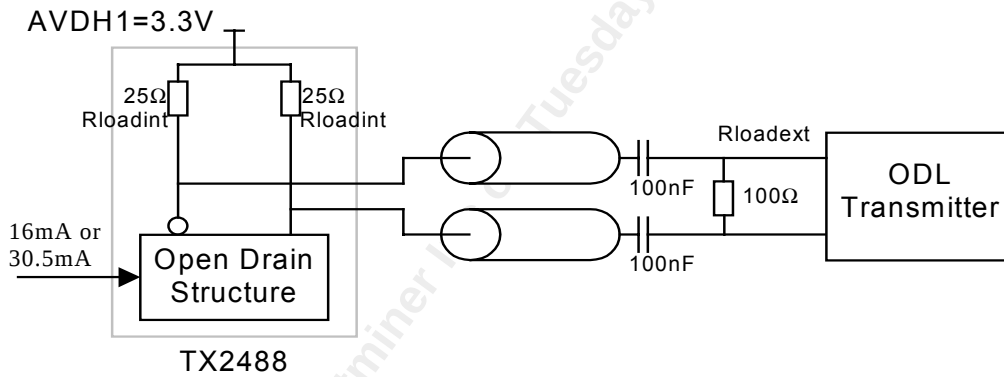
Figure 20 CRSU 4x2488 Tx Termination Scheme #2
