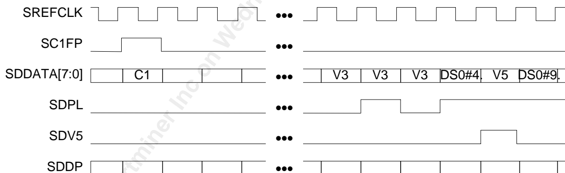
Figure 62 SBI DROP Bus T1/E1 Functional Timing
