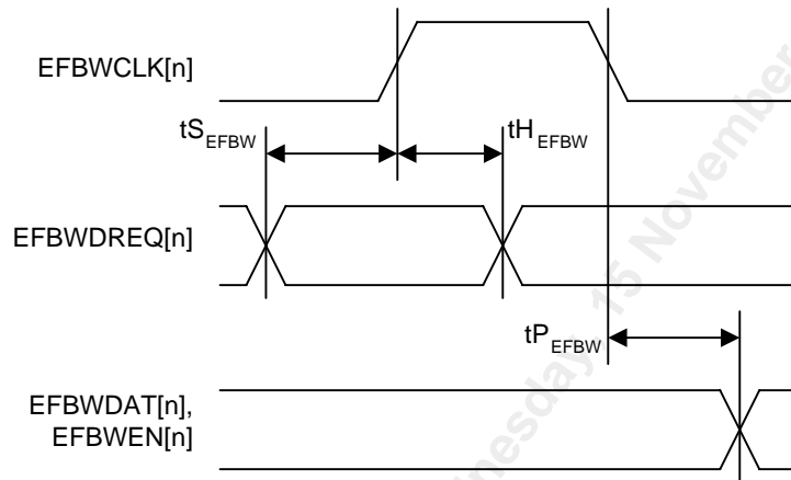
Figure 83 Egress Flexible Bandwidth Port Timing
