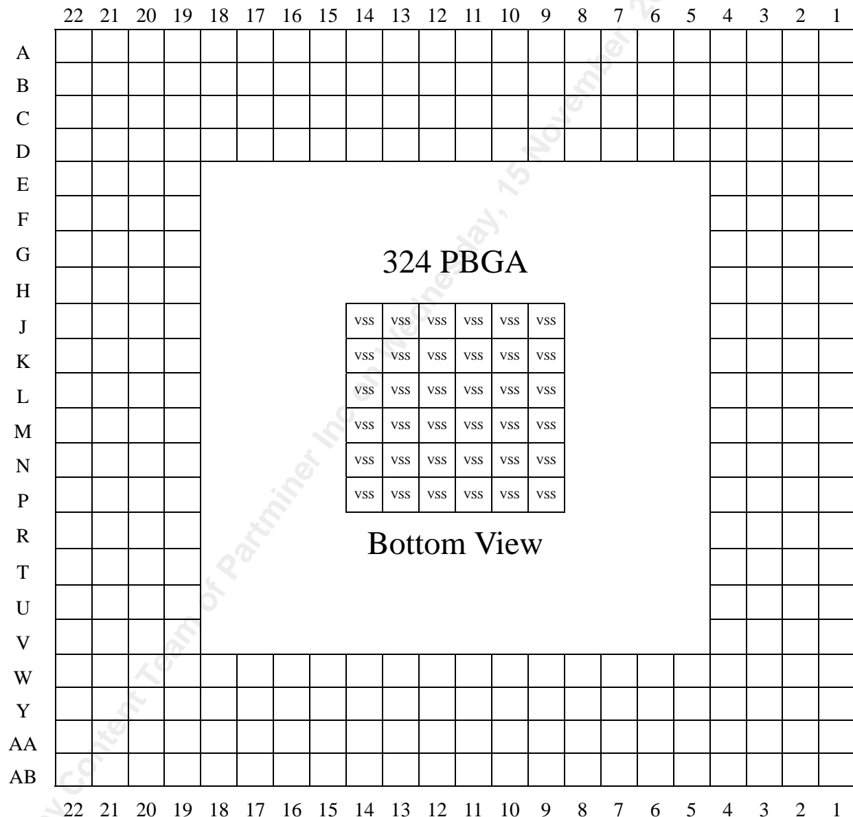
Figure 9 Pin Diagram
