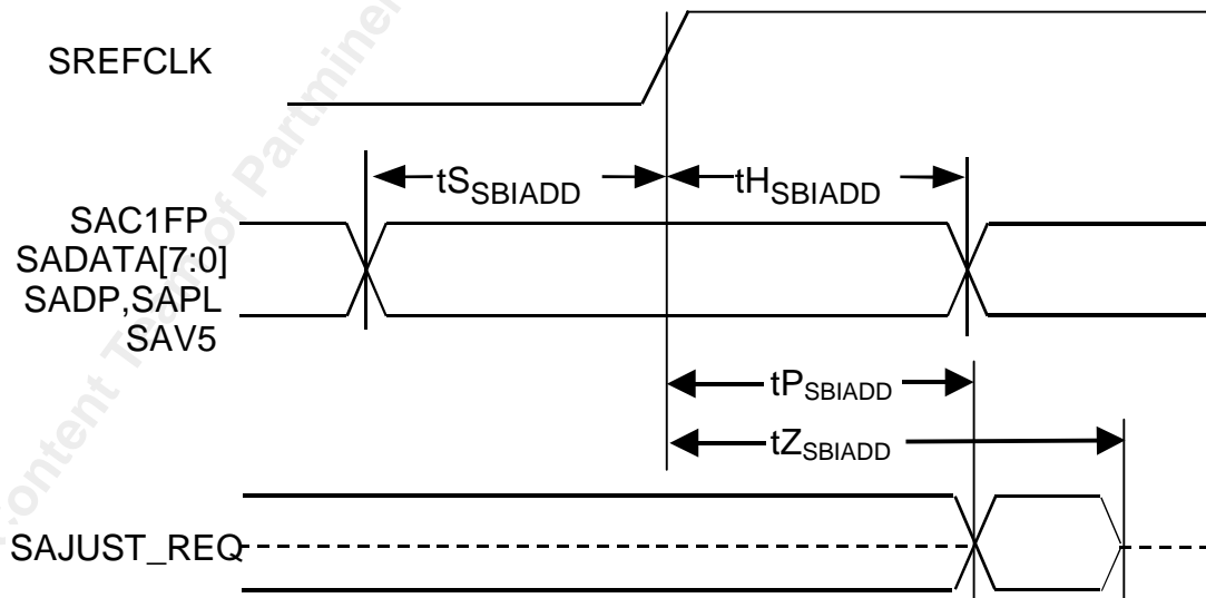
Figure 78 SBI ADD BUS Timing
