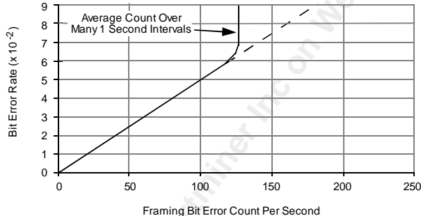
Figure 19 FER Count vs. BER (T1 ESF mode)
