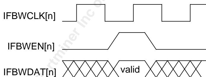
Figure 69 Ingress Flexible Bandwidth Port Functional Timing
