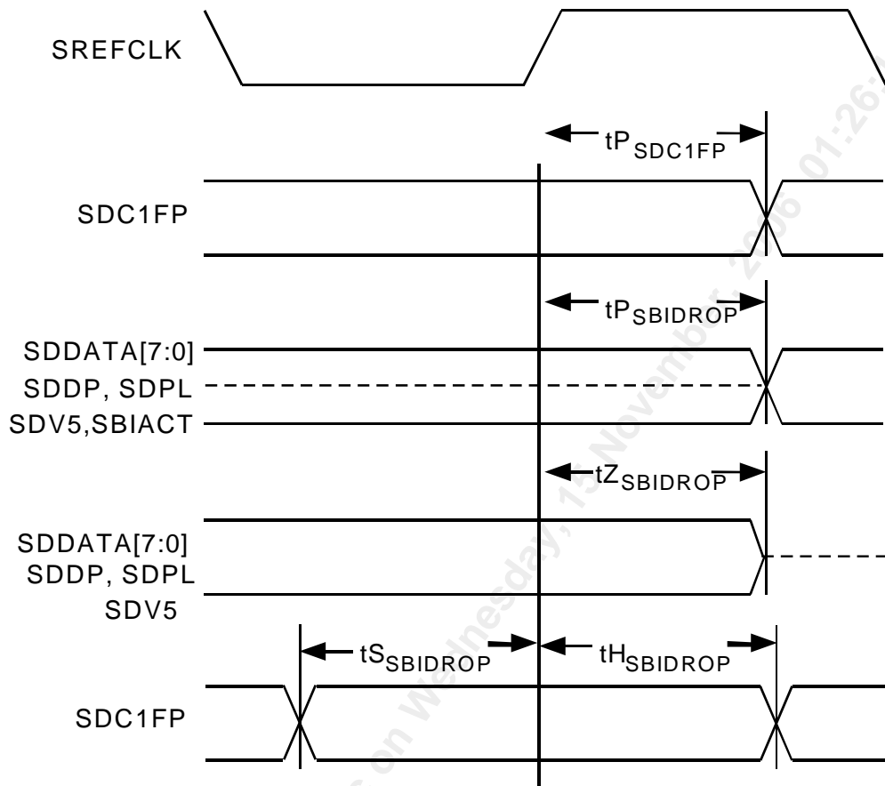
Figure 79 SBI DROP BUS Timing
