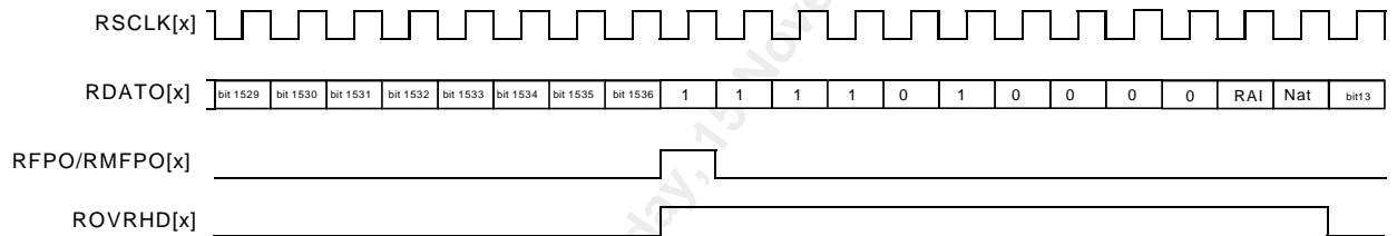
Figure 53 Framer Mode G.751 E3 Receive Output Stream with RGAPCLK
