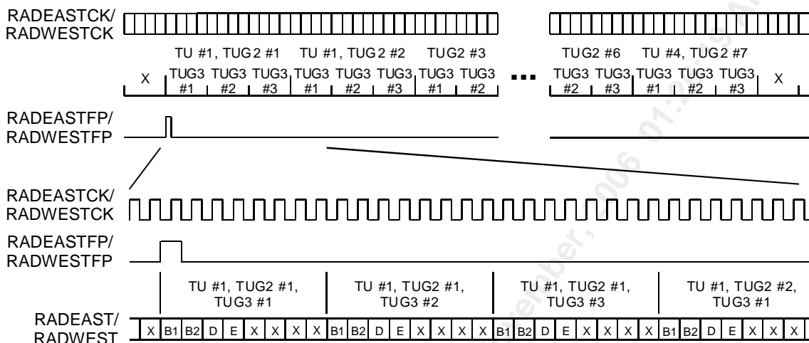
Figure 61 Remote Serial Alarm Port Timing
