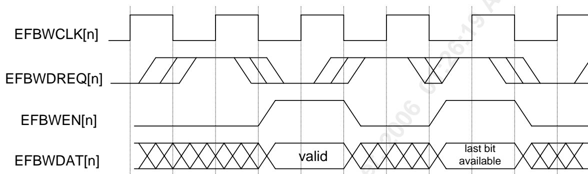
Figure 68 Egress Flexible Bandwidth Port Functional Timing SBI Master
