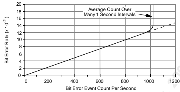
Figure 20 CRCE Count vs. BER (T1 SF mode)
