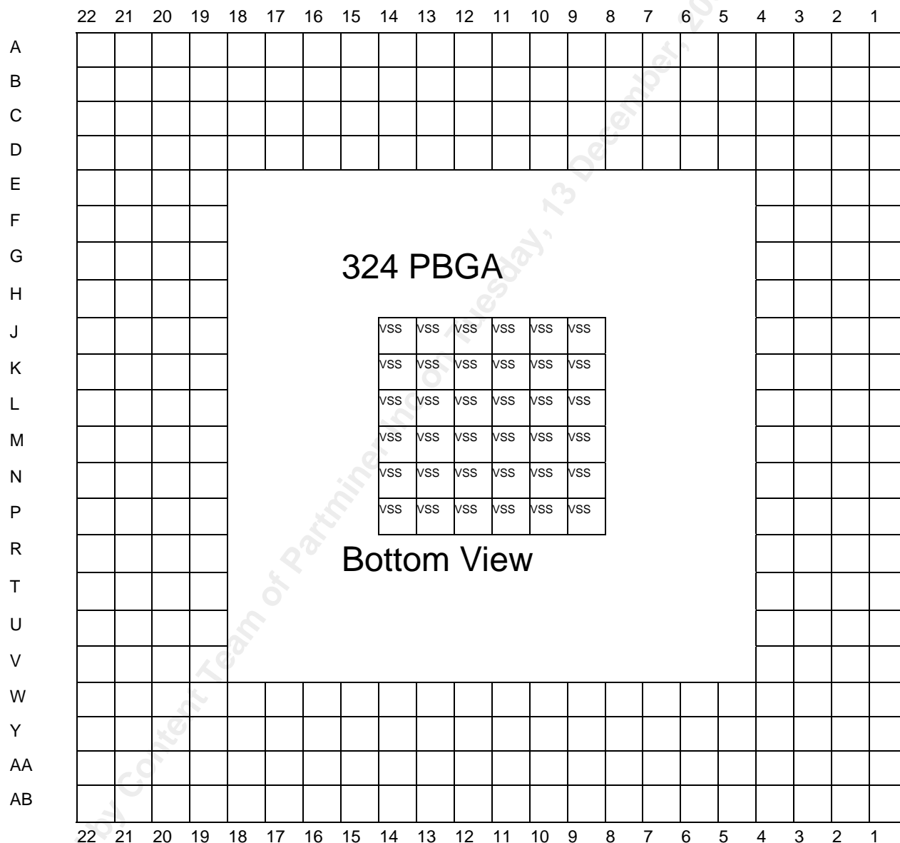
Figure 5 Pin Diagram
