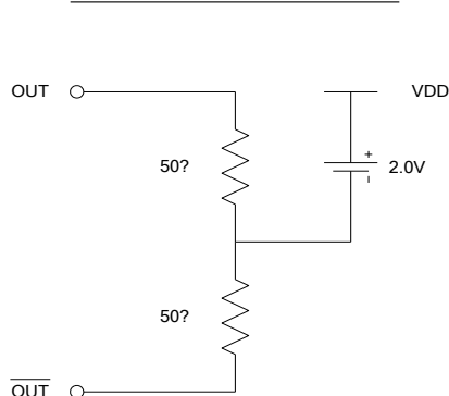
LVPECL Levels Test Circuit
