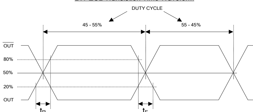
LVPECL Transistion Time Waveform
