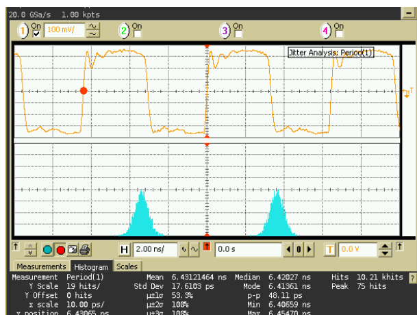
Figure 3: Period Jitter Histogram at 155.52 MHz Analog Frequency Multiplier (4x) with 38.88MHz crystal
