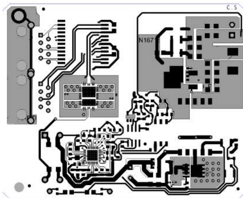
Figure 26: Top Layer
