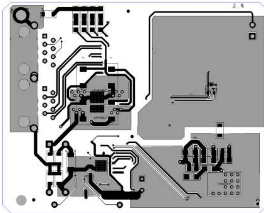
Figure 27: Bottom Layer
