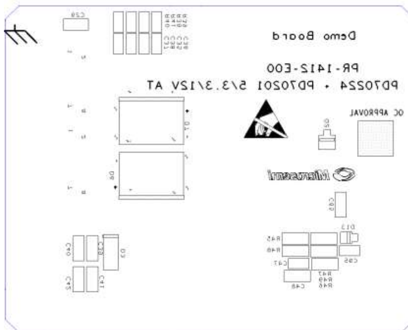
Figure 28: Bottom Silk
