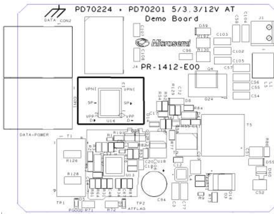
Figure 25: Top Silk
