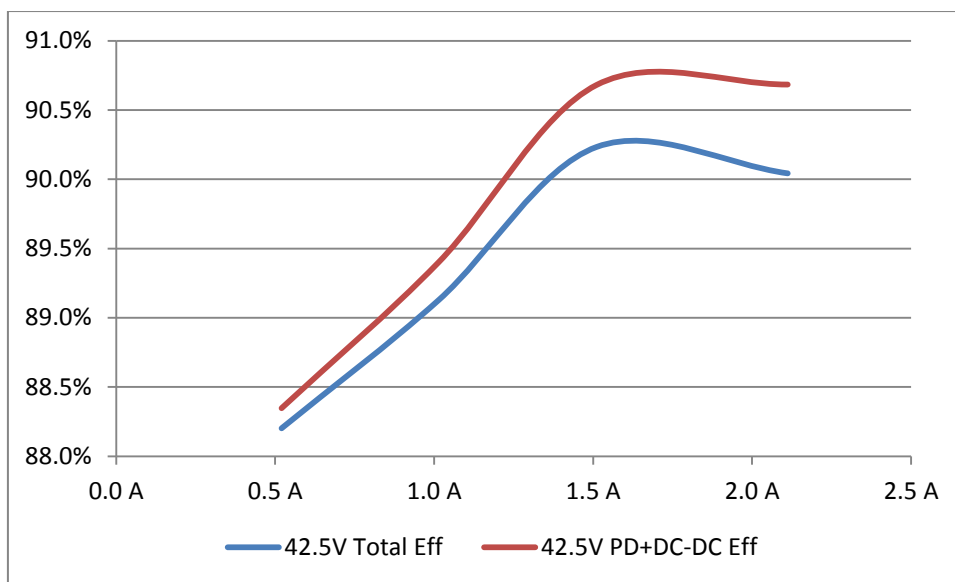
Figure 18: PD70201EVB25F12 Efficiency at 42.5V
