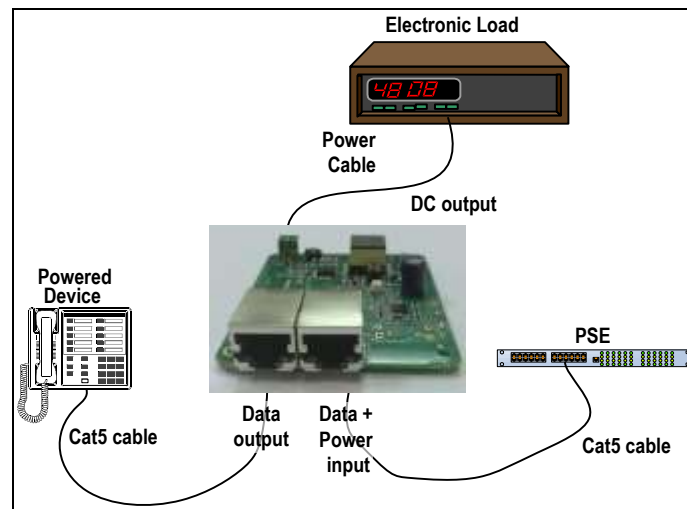
Figure 6: Test Setup
