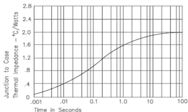
FIGURE 4 TRANSIENT THERMAL IMPEDANCE
