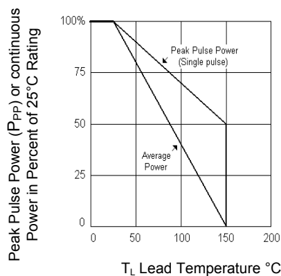
FIGURE 3 Derating Curve
