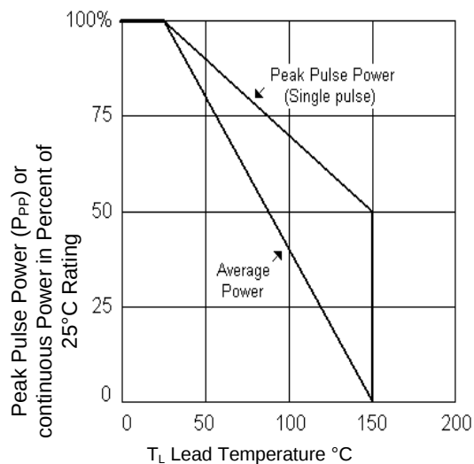
FIGURE 3: Derating Curve
