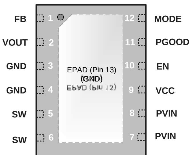
LX7157B DFN 3.5mm x 3mm 12L Top View
