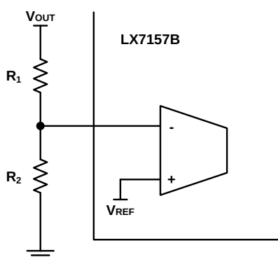
Figure 5: Voltage Divider
