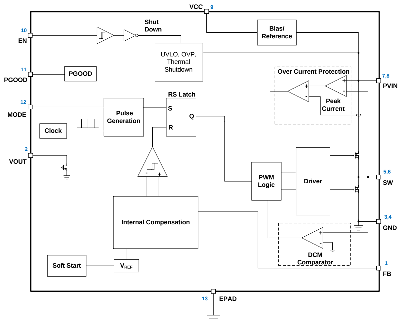
Figure 3: Block Diagram
