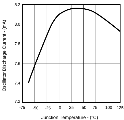
Figure 9 • Oscillator Discharge Current vs. Temperature
