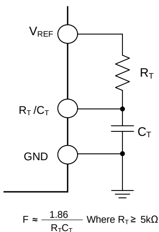
Figure 13 • Oscillator Timing Circuit
