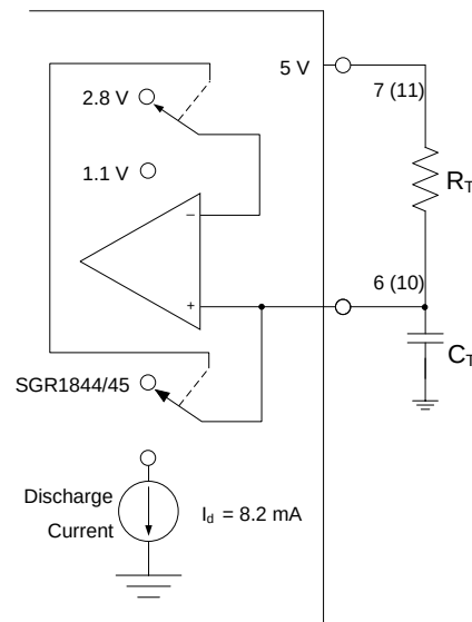
Figure 21 • Oscillator Connection
