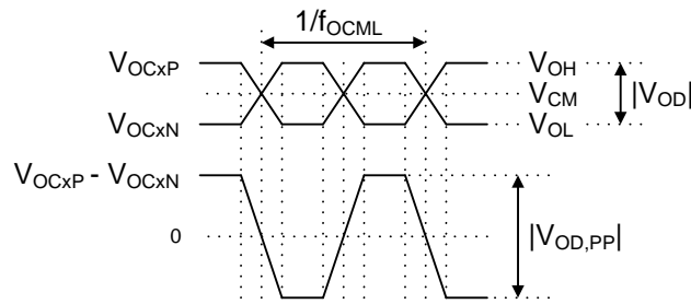
Figure 17 - Electrical Characteristics: CML Clock Outputs
