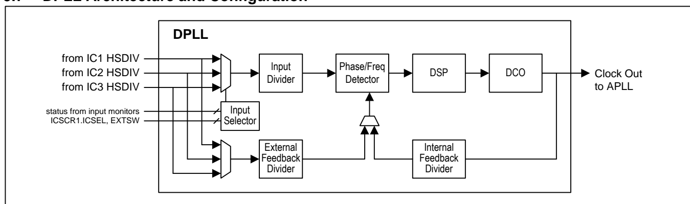
Figure 5 - DPLL Block Diagram
