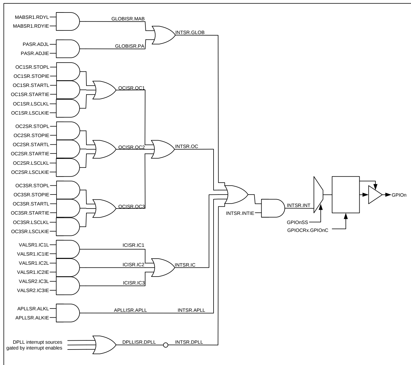
Figure 14 – Interrupt Structure
