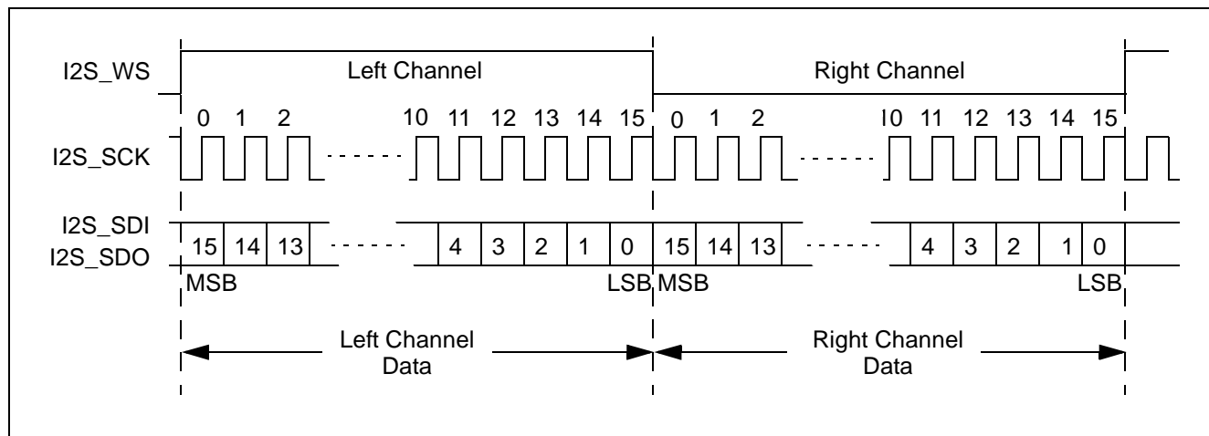
Figure 10 - Left Justified Mode
