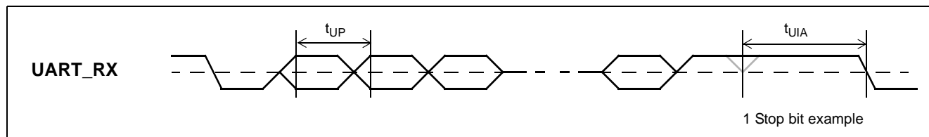
Figure 43 - UART_RX Timing
