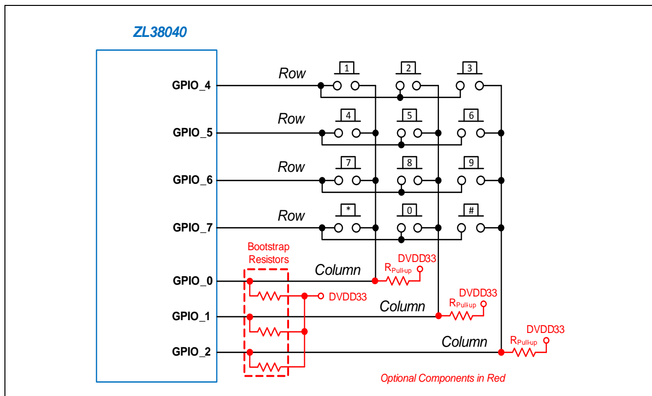
Figure 25 - A 3x4 Keypad Array Implementation
