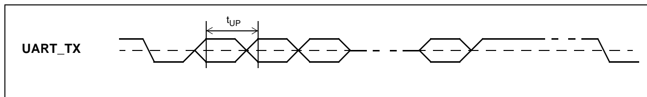
Figure 44 - UART_TX Timing
